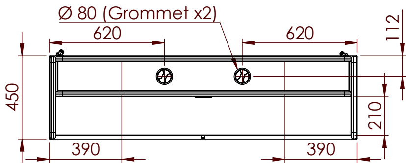
Bottom view cable channel
