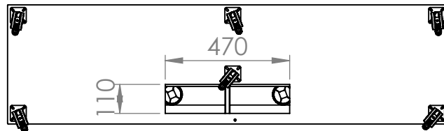
Bottom view cable channel
